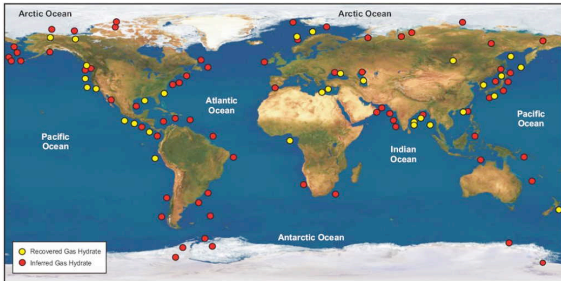
Fig. 2: Inferred and recovered gas hydrate locations [2]. Estimates of world NGH deposits, ranging from 2.5 \times 10^{15} \text{ m}^3 to 3.0 \times 10^{18} \text{ m}^3 , show that the amount of organic carbon contained in NGH reservoirs is twice the amount contained in all currently recoverable worldwide conventional hydrocarbon resources.
